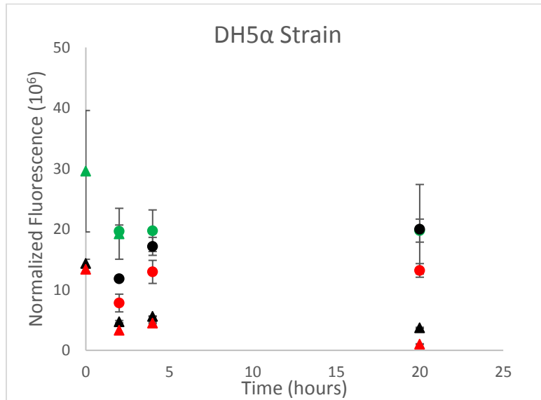
Figure 1. The positive control pTrc-GFP plasmid (green), experimental FNR-GFP plasmid (black) and the negative control that does not contain a plasmid (red) were all tested in the DH5α strain and normalized fluorescence is shown. The triangular markers represent aerobic conditions and the circular markers represent anaerobic conditions. Each error bar represents one standard deviation.
