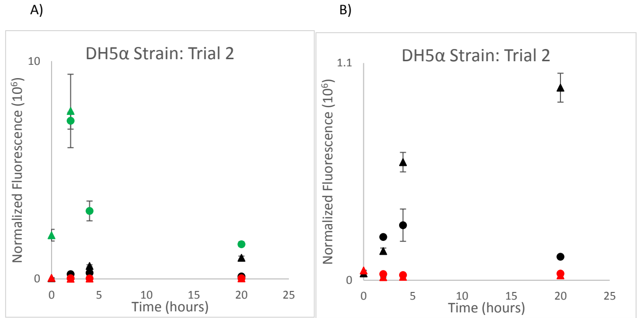
Figure 2. The positive control pTrc-GFP plasmid (green), experimental FNR-GFP plasmid (black) and the negative control that does not contain a plasmid (red) were all tested in the DH5α strain and normalized fluorescence is shown. The triangular markers represent aerobic conditions and the circular markers represent anaerobic conditions. The fluorescence expression during this trial was measured using an excitation wavelength of 485 nm and an emission wavelength of 520 nm. The data points for the aerobic conditions of the positive controls at 4 and 20 hours do not appear on this graph because the plate reader reached saturation under the medium sensitivity setting used. The graph on the right (B) shows just the FNR-GFP plasmid and the negative control on a smaller scale. Each error bar represents one standard deviation.
