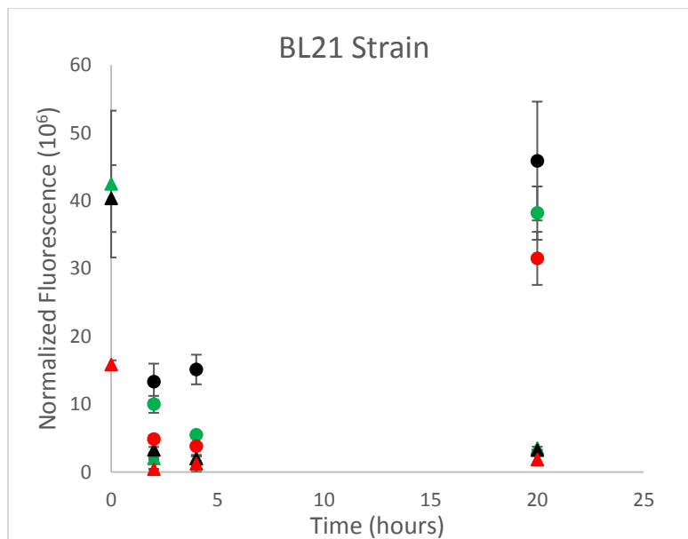
Figure 4. The positive control pTrc-GFP plasmid (green), experimental FNR-GFP plasmid (black) and the negative control that does not contain a plasmid (red) were all tested in the BL21 strain and normalized fluorescence is shown. The triangular markers represent aerobic conditions and the circular markers represent anaerobic conditions. Each error bar represents one standard deviation.
