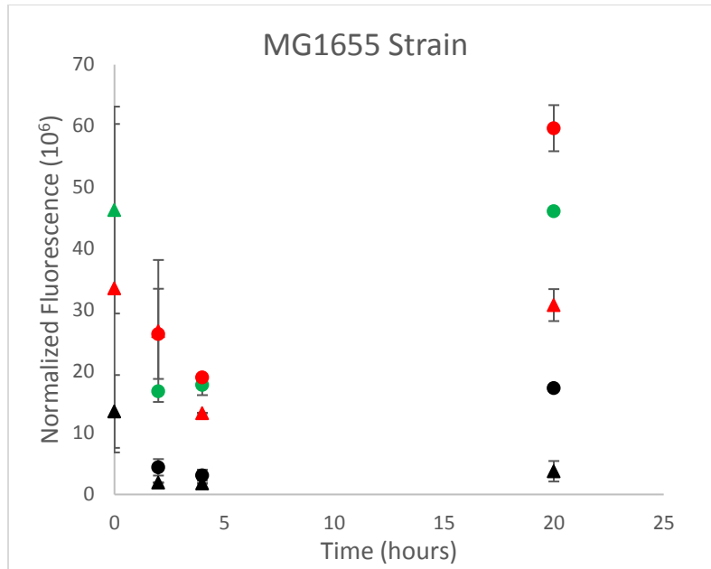
Figure 3. The positive control pTrc-GFP plasmid (green), experimental FNR-GFP plasmid (black) and the negative control that does not contain a plasmid (red) were all tested in the MG1655 strain and normalized fluorescence is shown. The triangular markers represent aerobic conditions and the circular markers represent anaerobic conditions. Each error bar represents one standard deviation.
