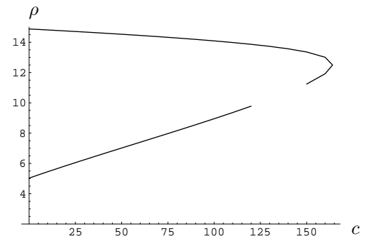
Figure 5.4: \rho vs. c such that \tilde{G}(\rho, c) = 0 with a = 15 and b = 3
