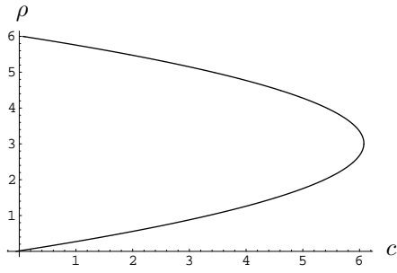
Figure 4.5: \rho vs. c such that \tilde{G}(\rho, c) = 0 with a = 15
