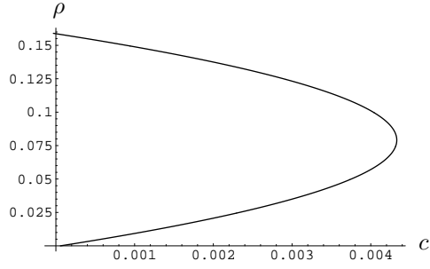
Figure 4.3: \rho vs. c such that \tilde{G}(\rho, c) = 0 with a = 10
