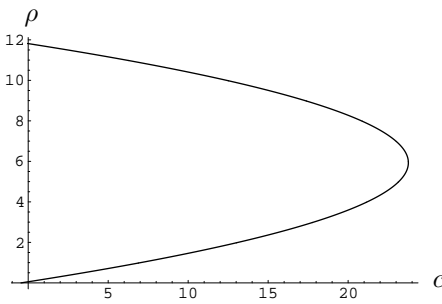
Figure 4.7: \rho vs. c such that \tilde{G}(\rho, c) = 0 with a = 20
