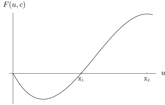
Figure 4.1: General shape of F(u, c)
