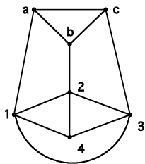
Figure 7: The graph R_7
