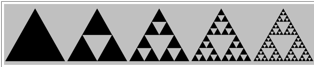
The first four stages of removal of the Sierpinski triangle
