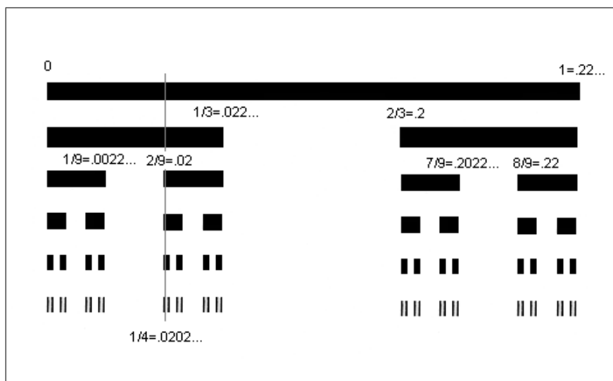
Five stages of removal of the Cantor Ternary Set
