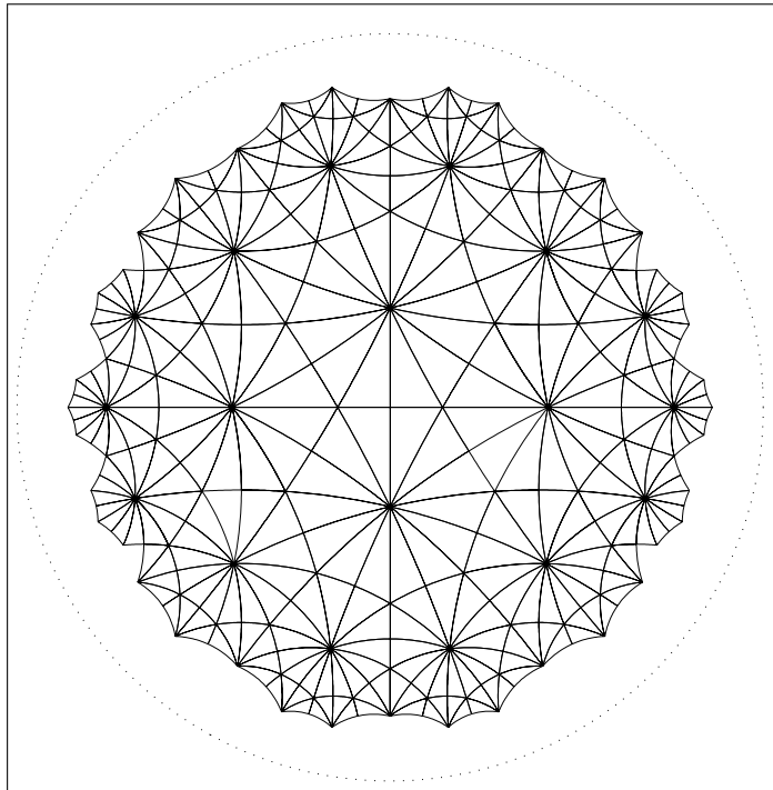
Figure 3. A portion of the (2, 3, 7) tiling
