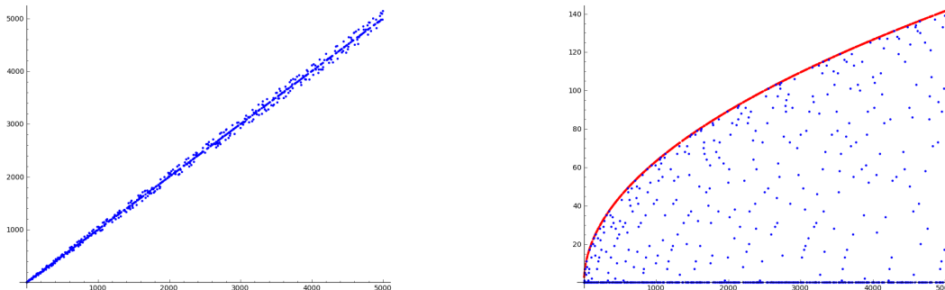
(a) The points (p, |E(\mathbb{F}_p)|) for the first 5000 primes showing roughly 1:1 correspondence as expected. (b) The points (p, |E(\mathbb{F}_p) - p - 1|) under the curve 2\sqrt{p} in red.
