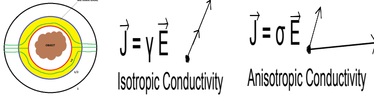
Figure 3: Anisotropic conductivity is needed in the metamaterial as shown in the yellow region.
